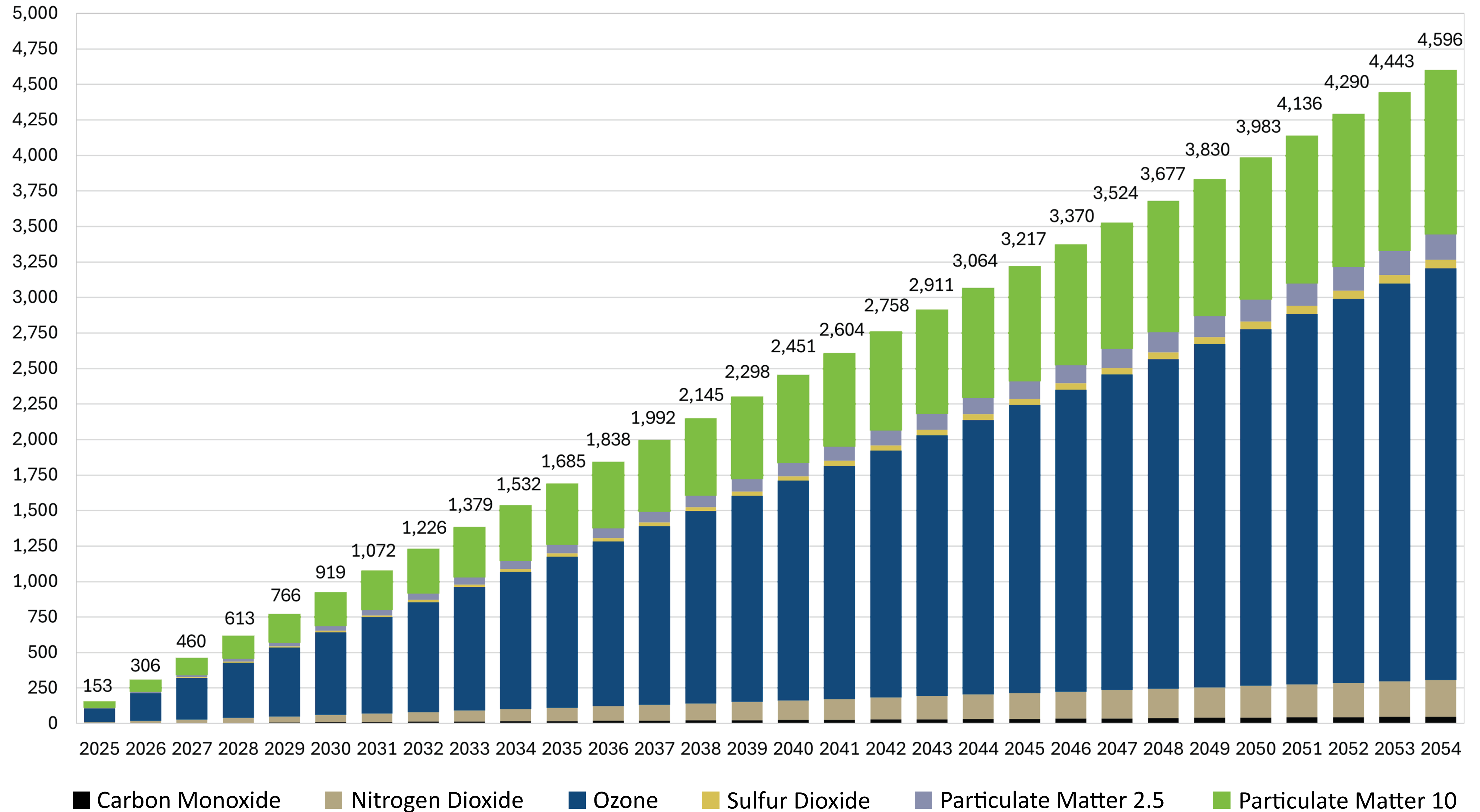
Figure 2 Cumulative Air Pollution Removals over 30 Years.
